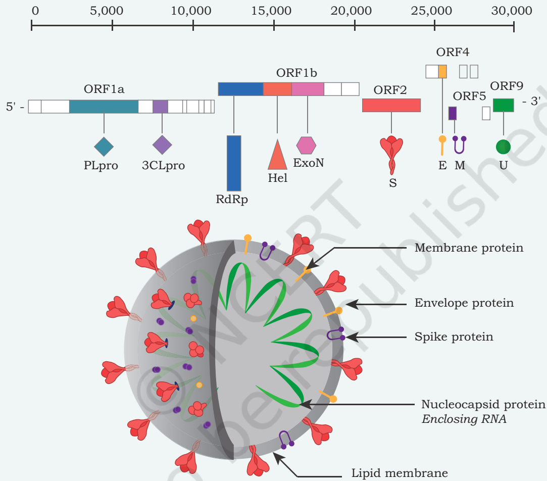
Schematic diagram of the SARS-CoV-2 genome organisation and a virion. The genome contains a 5'-untranslated region (5'-UTR), open-reading frames (ORFs) 1a and 1b encodes non-structural proteins, 3-chymotrypsin-like protease (3CLpro), papain-like protease (PLpro), helicase (Hel), and RNA-dependent RNA polymerase (RdRp) besides accessory proteins, The other ORFs code for structural S protein (S), E protein (E), M protein (M), and N phosphoprotein (N).
