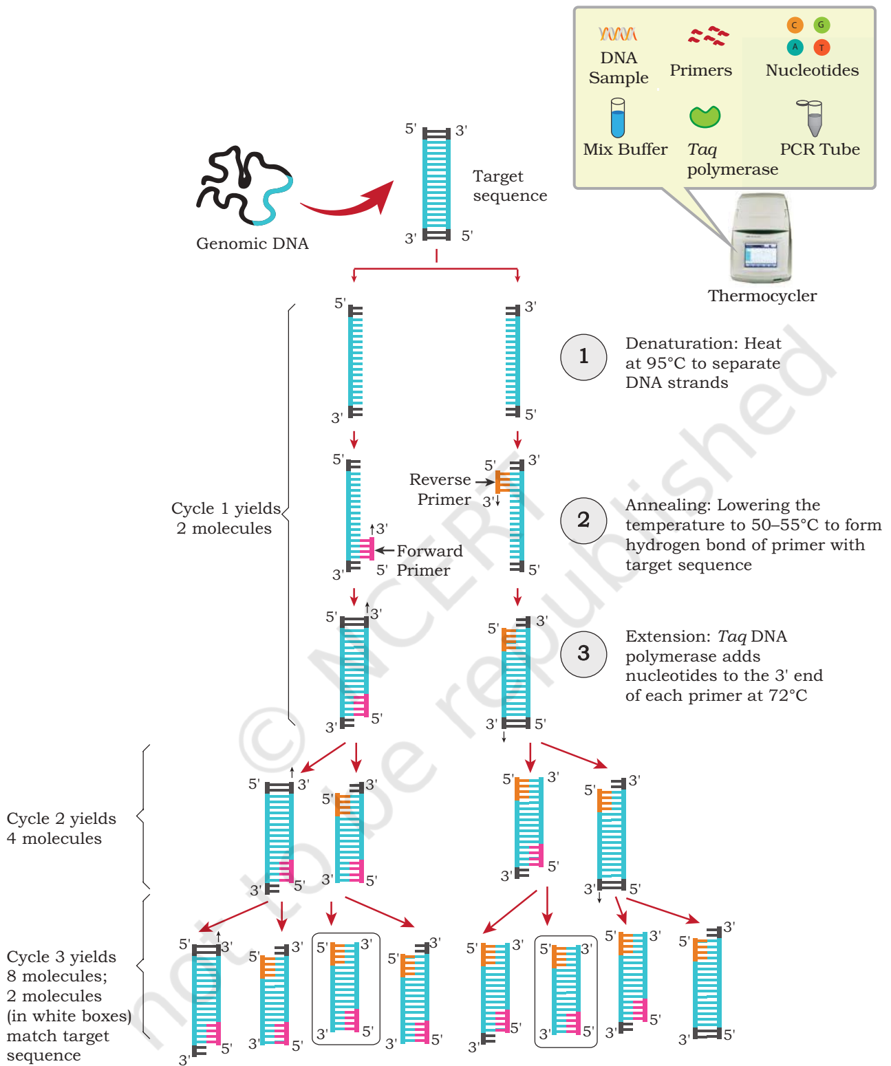
Fig. 3.18: Steps of polymerase chain reaction
