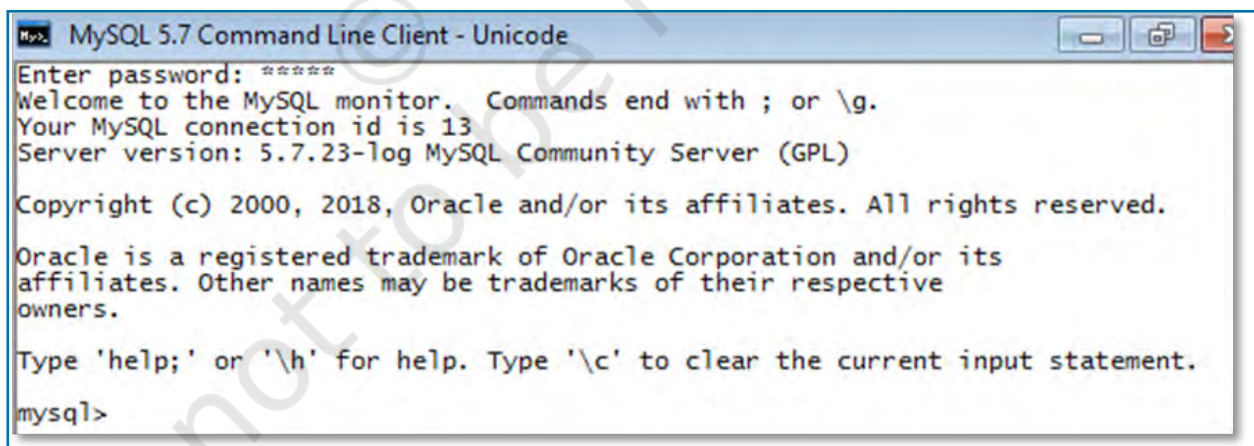
Figure 9.1: MySQL Shell
